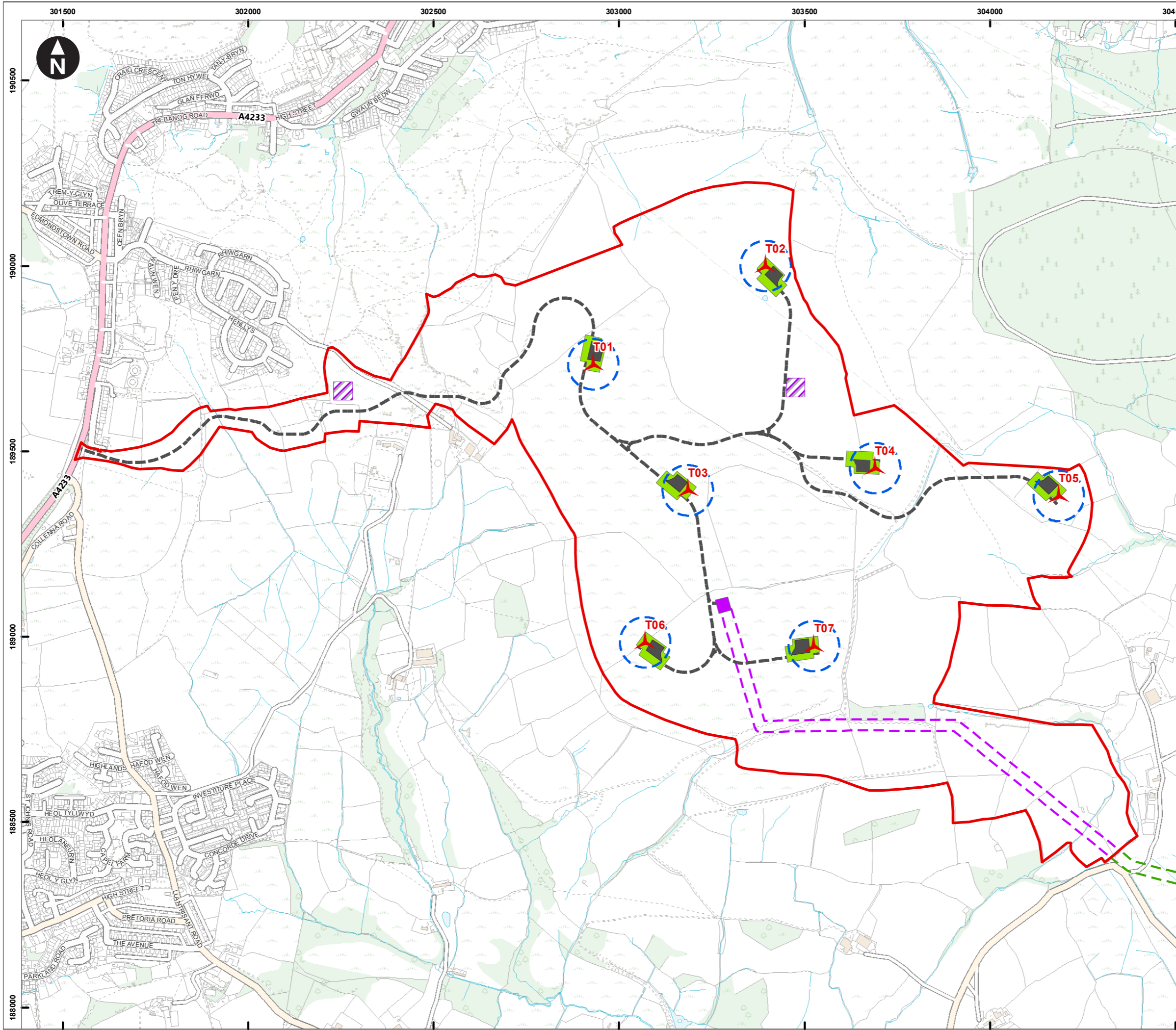
Figure 10.1a Wind farm development - site layout
