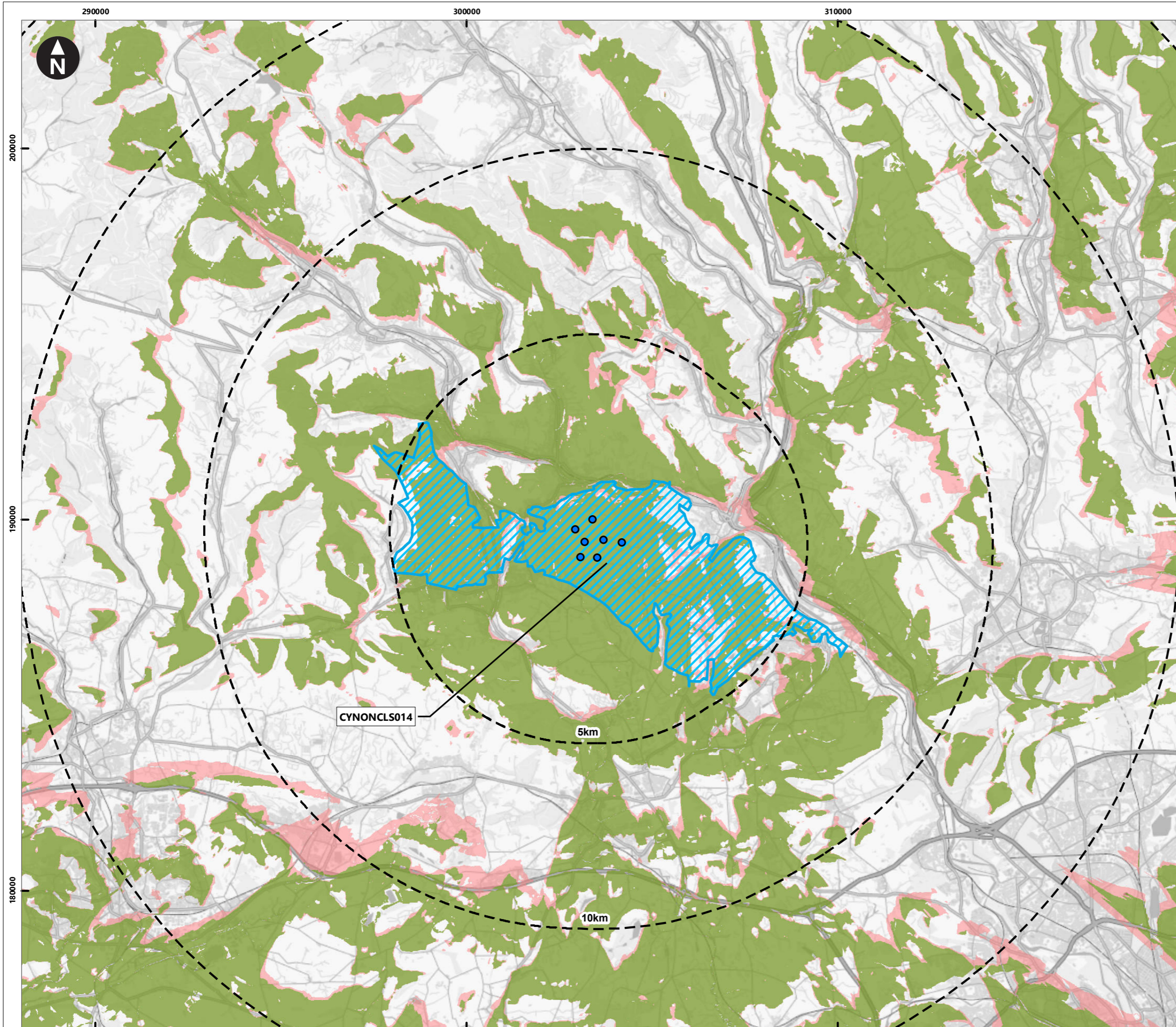
Figure 6.11 LANDMAP: Cultural Landscape Services Aspect Areas filtered into the Study Area with Zone of Theoretical Visibility (ZTV) to Hub and Blade Tip
