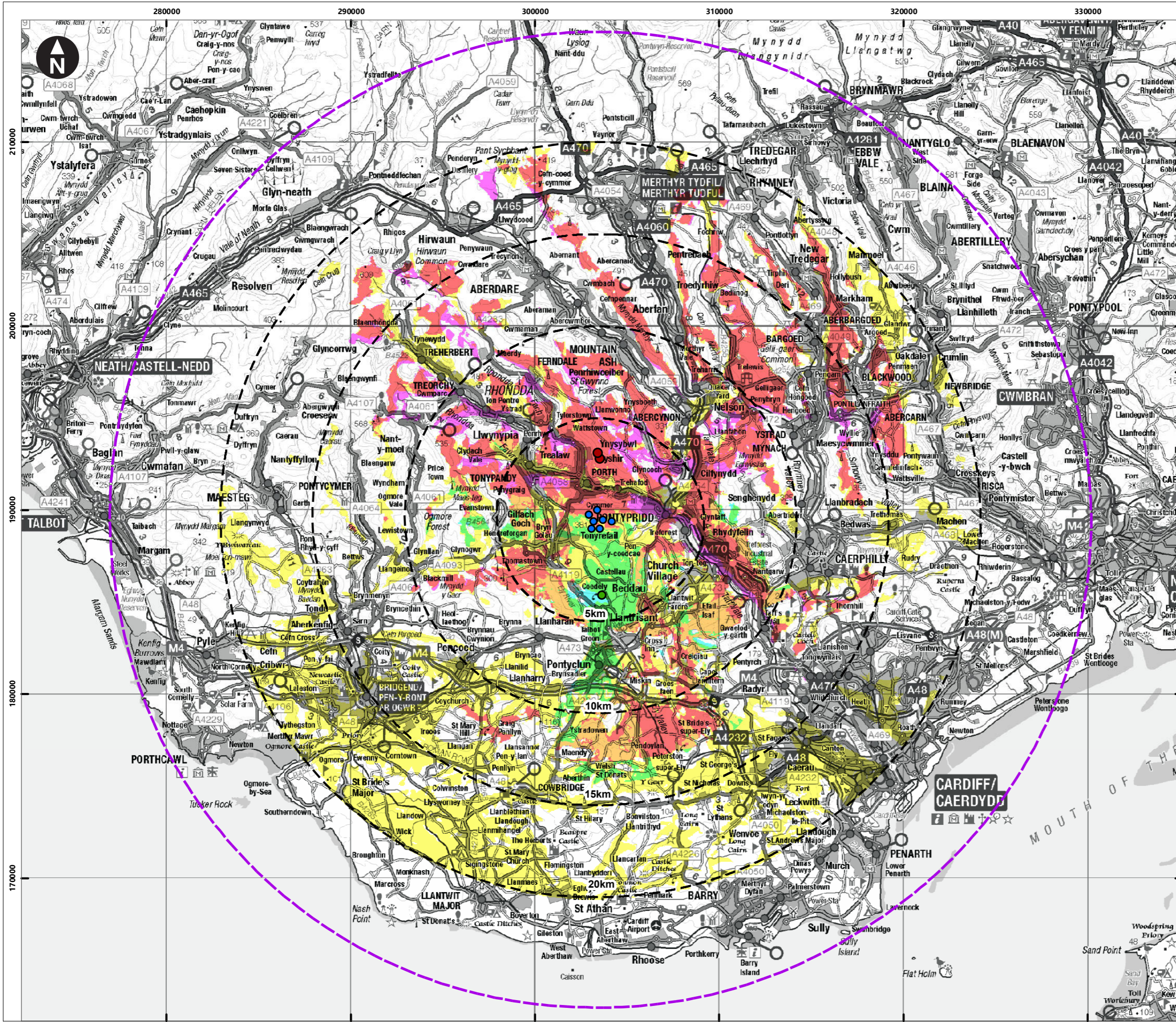
Figure 6.20 Cumulative Zones of Theoretical Visibility in relation to West of Rhiwefelin Farm and Llwyncelyn Farm wind turbines
